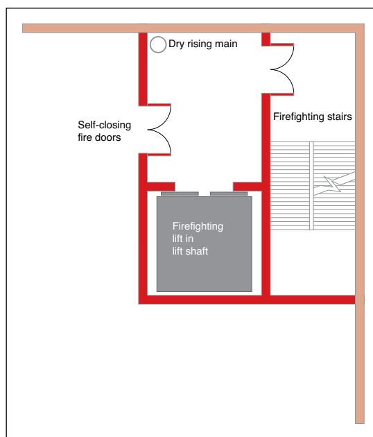
Figure 19: Firefighting shaft
