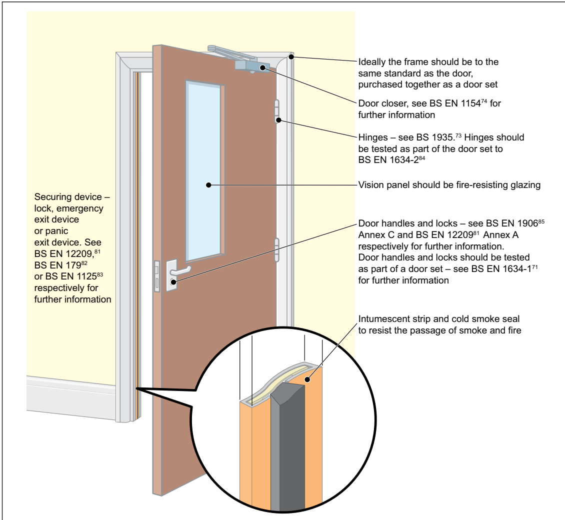
Figure 61: A fire-resisting and smoke stopping door
