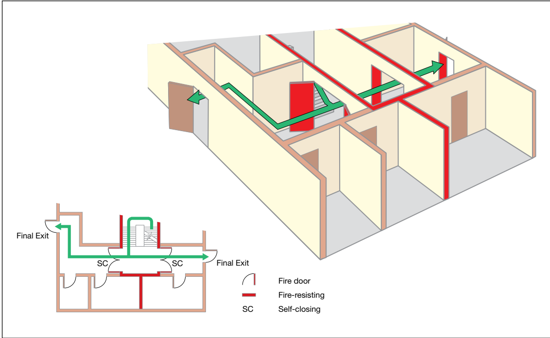
Figure 36: Example of two escape routes from a protected stairway to final exits
