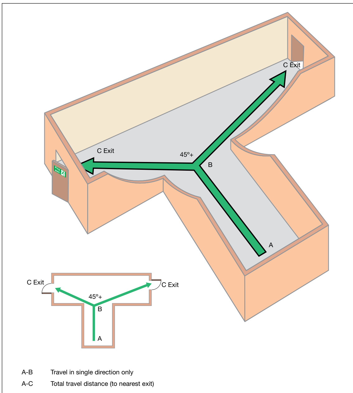
Figure 27: Measuring travel distance from initial dead end (open plan)
