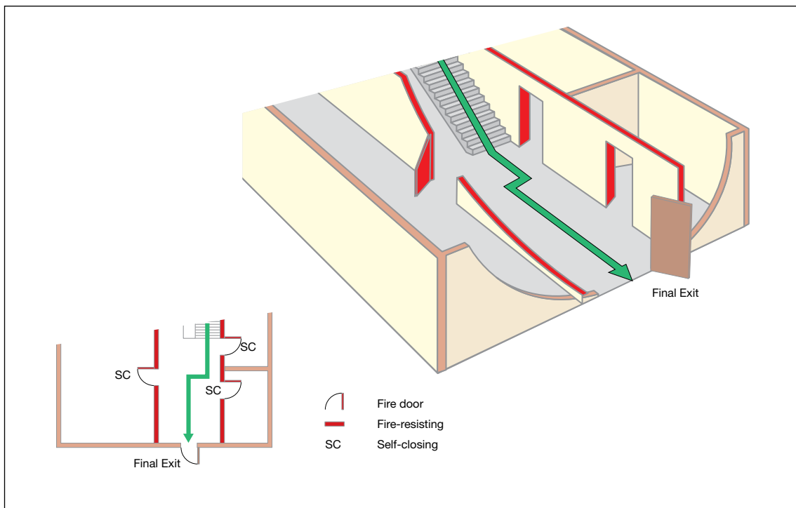
Figure 35: Examples of a protected route from a stairway to a final exit
