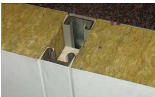
Figure 16: Insulated core panels - internal
