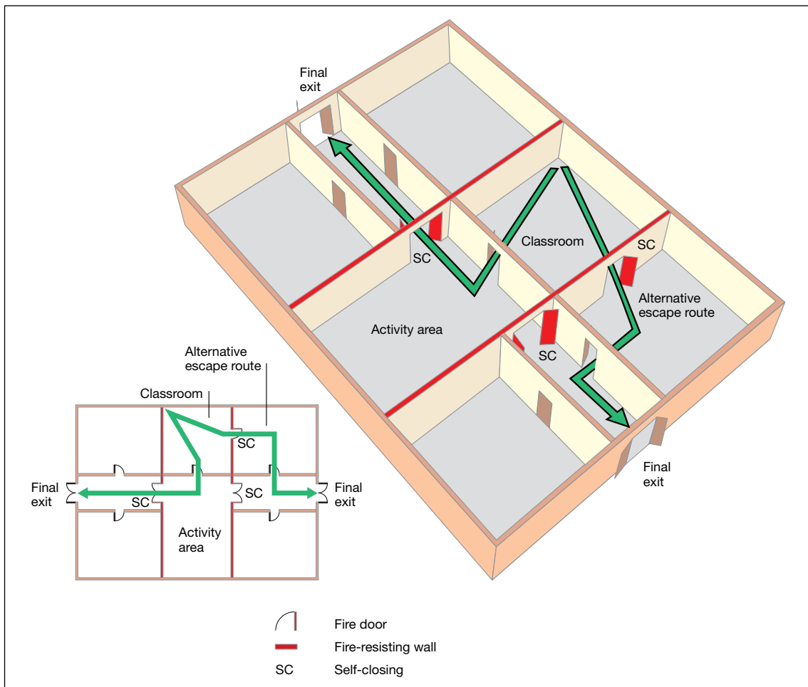
Figure 44: Ground floor with alternative escape route to bypass an activity area
