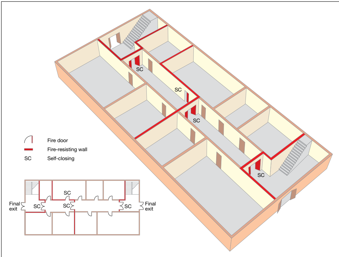
Figure 37: Separation of protected stairways
