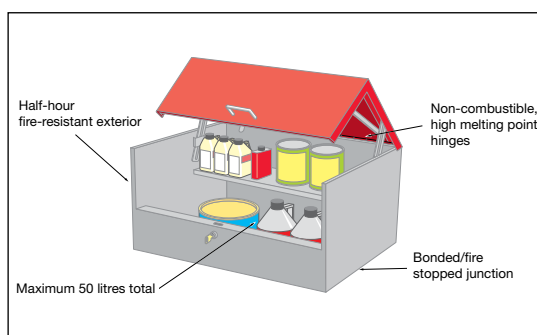
Figure 15: A 50-litre storage bin for flammables
