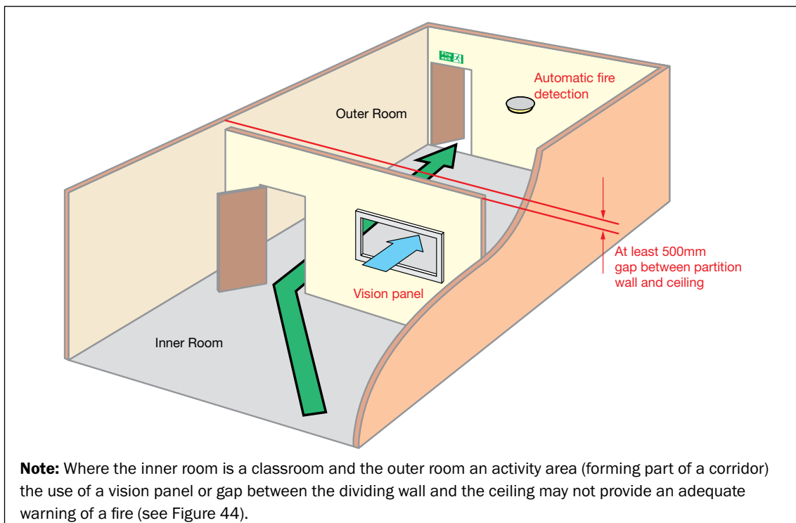
Figure 24: Inner rooms
