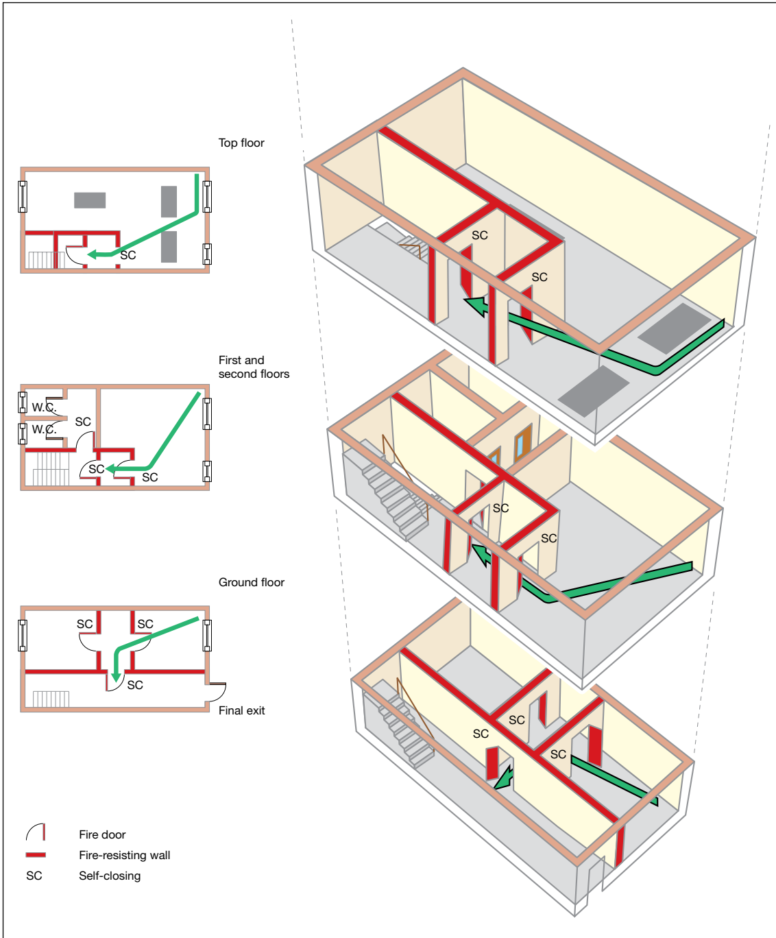
Figure 50: Four storey, ground and up to three upper floors protected by lobbies/corridors
