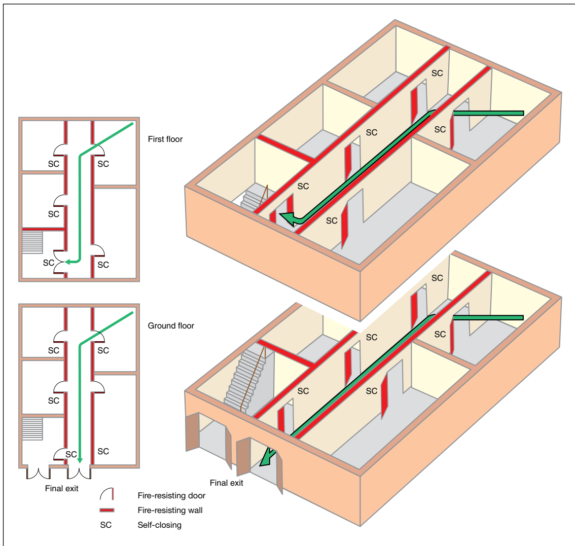
Figure 49: Two storey, ground and first floor
