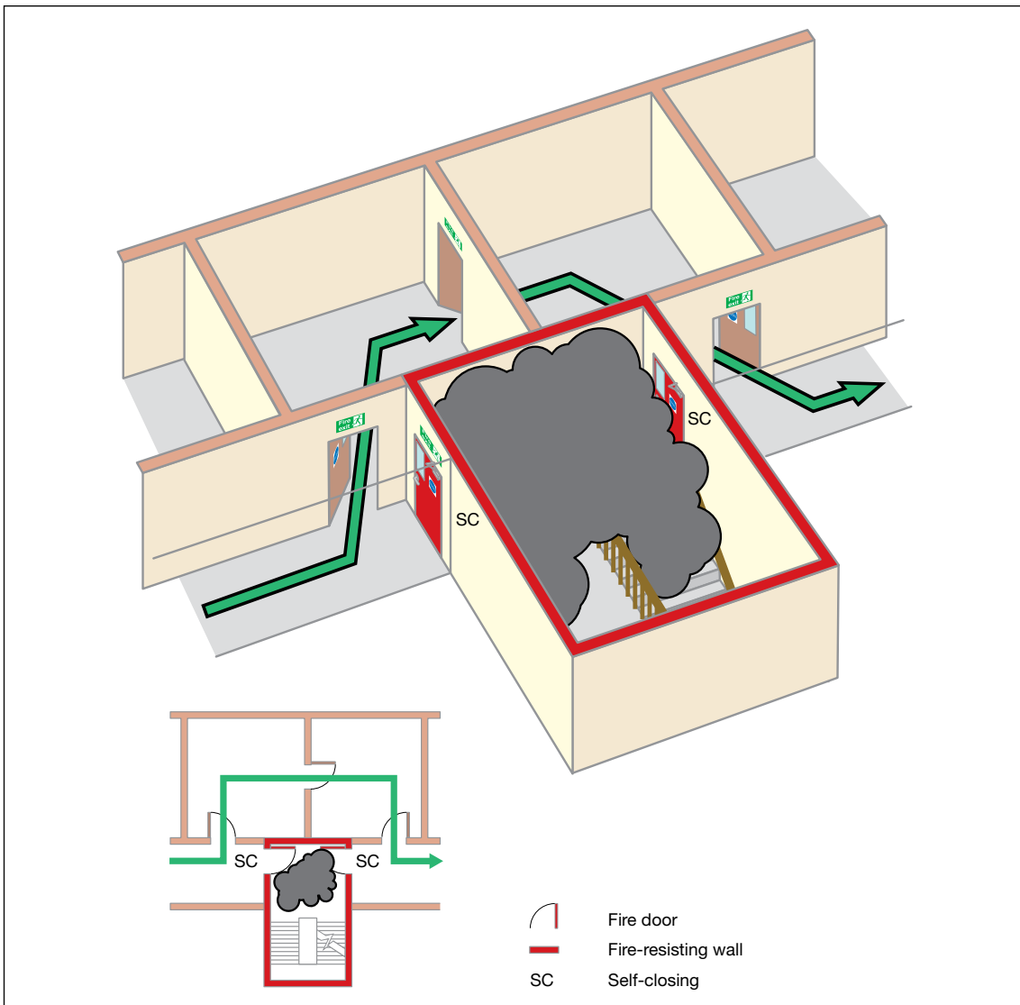
Figure 38: A stairway bypass route
