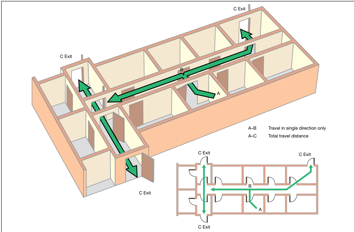
Figure 31: Dead-end condition provided with an alternative exit
