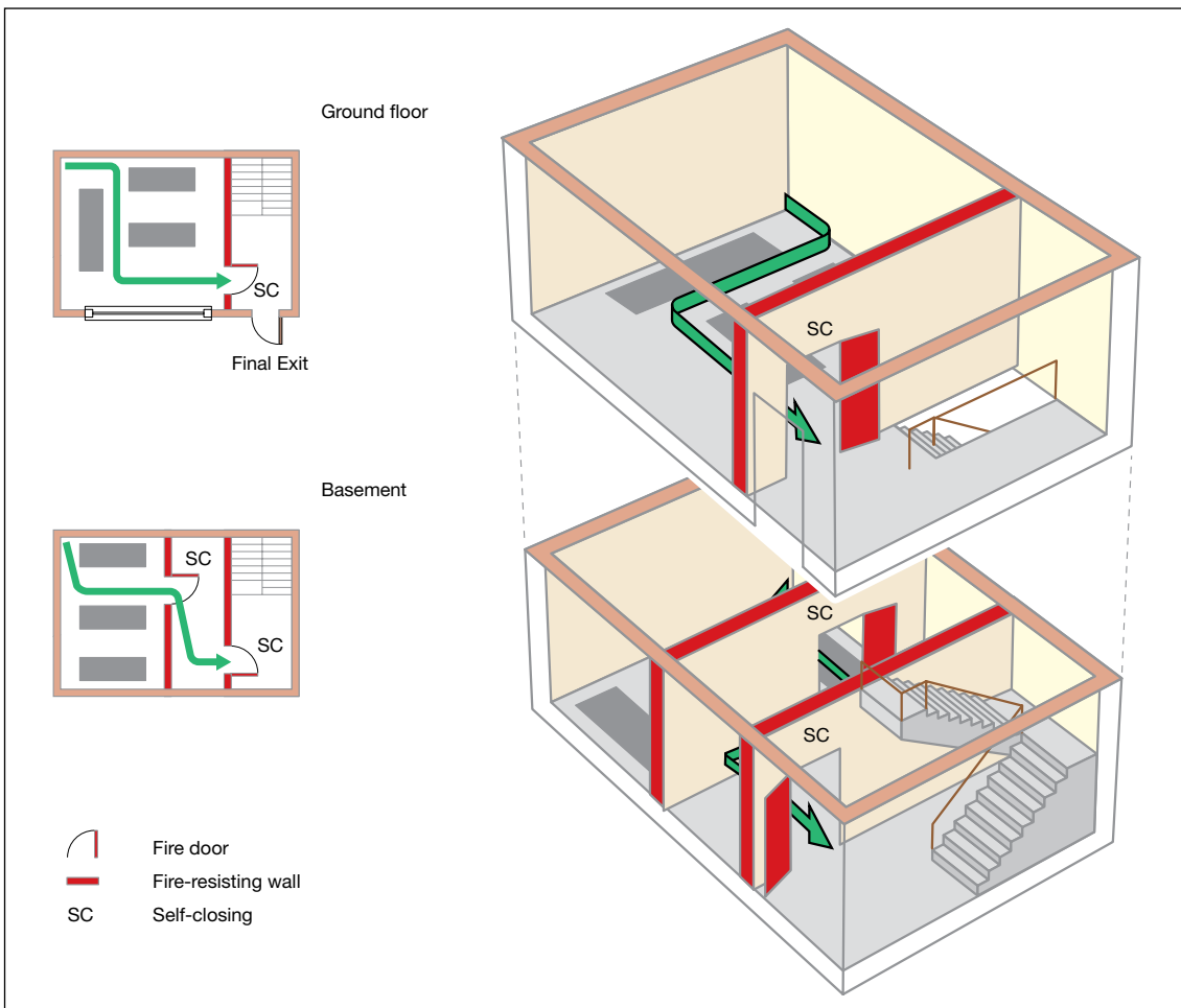
Figure 48: Two storey, basement and ground floor
