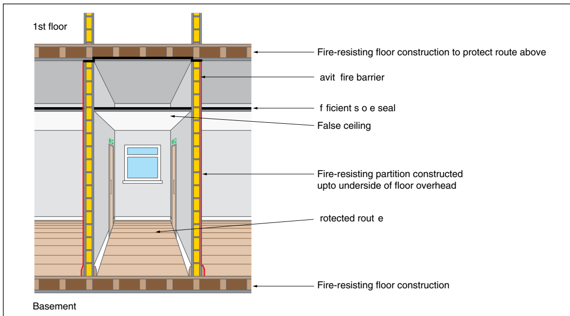
Figure 60: Fire-resisting construction
