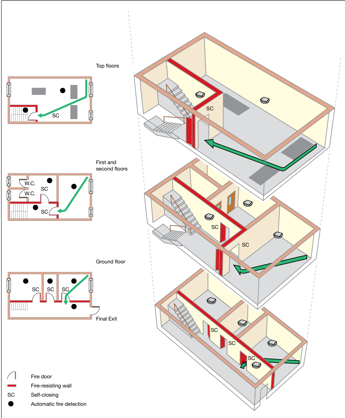
Figure 51: Four-storey premises: ground and up to three upper floors – protected with automatic fire detection
