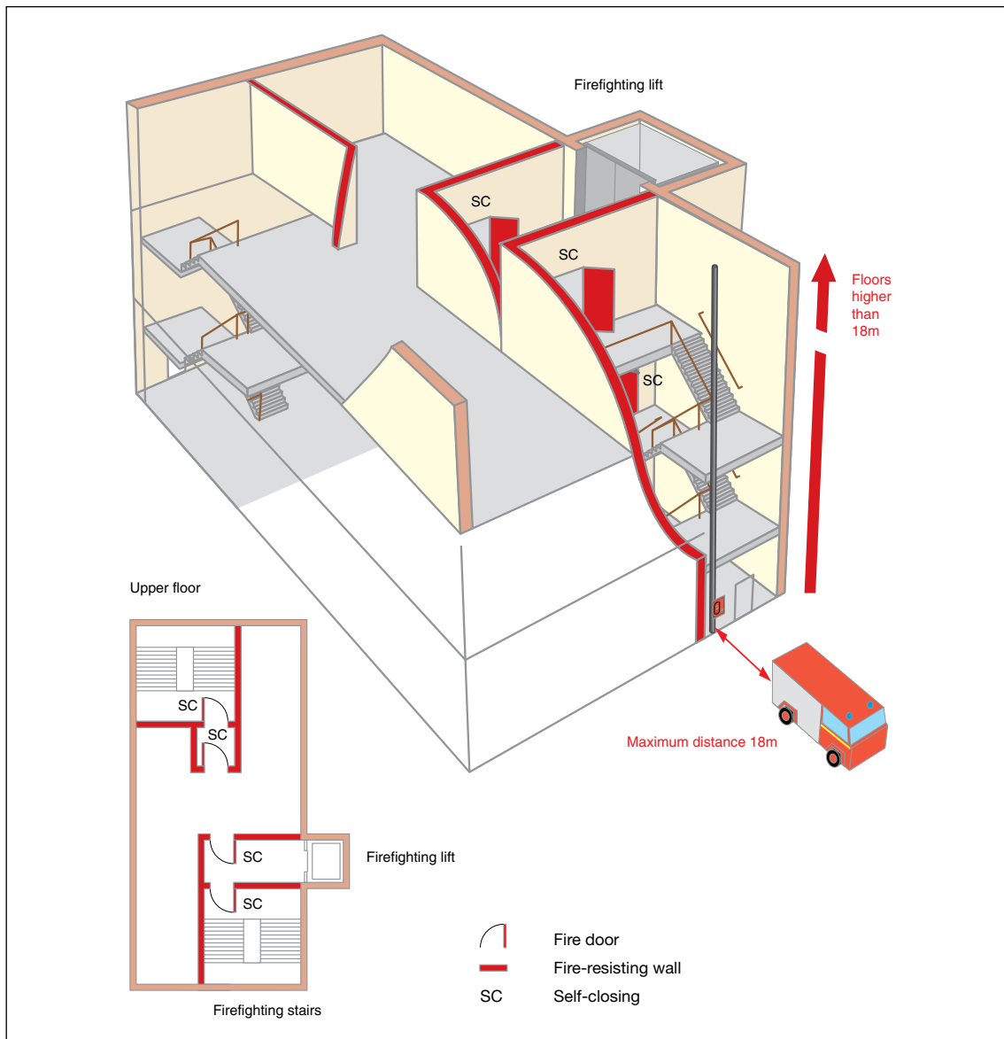
Figure 47: Tall building with a firefighting shaft
