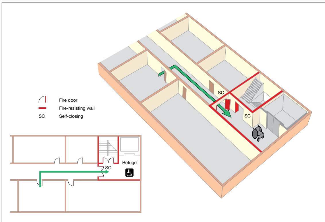
Figure 21: An example of a refuge
