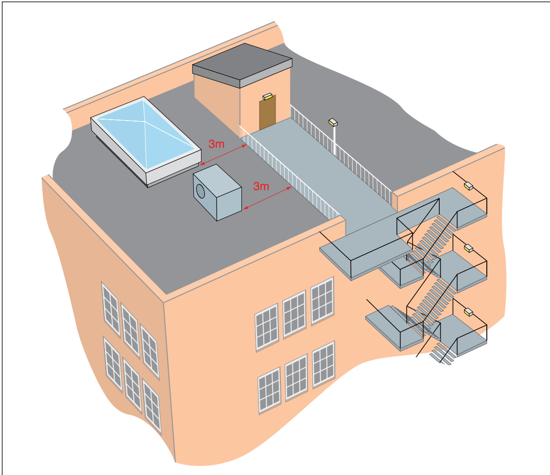
Figure 40: An escape route across a roof
