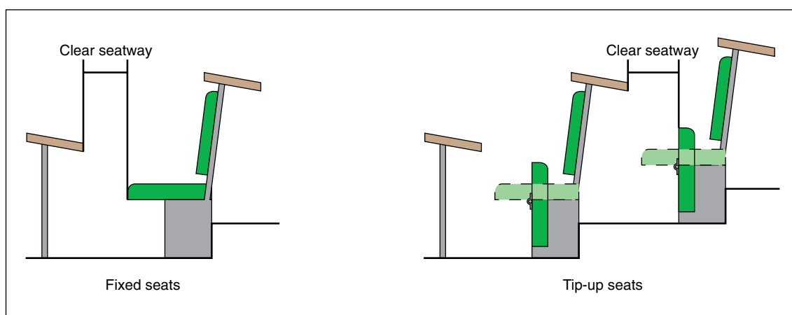
Figure 22: Clear space between seating
