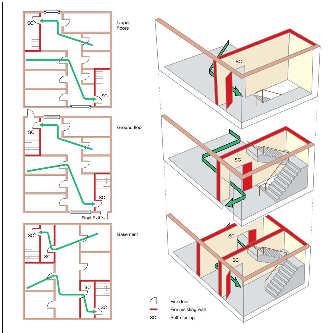
Figure 46: Basement, ground and up to three upper storeys
