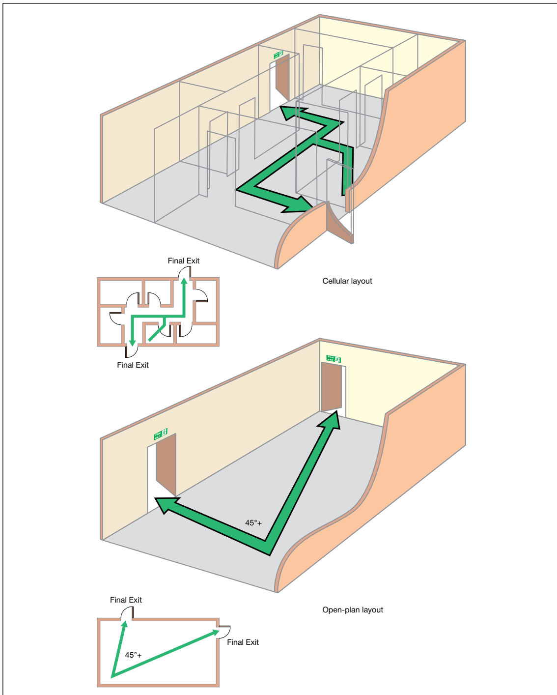
Figure 42: Ground floor with more than one exit (cellular and open plan)
