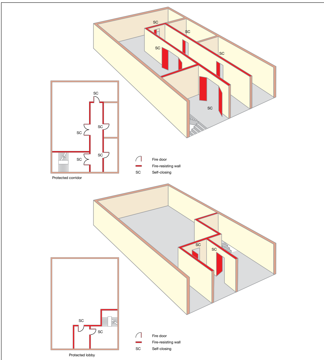
Figure 34: Examples of a Stairway with protected lobby/corridor approach
