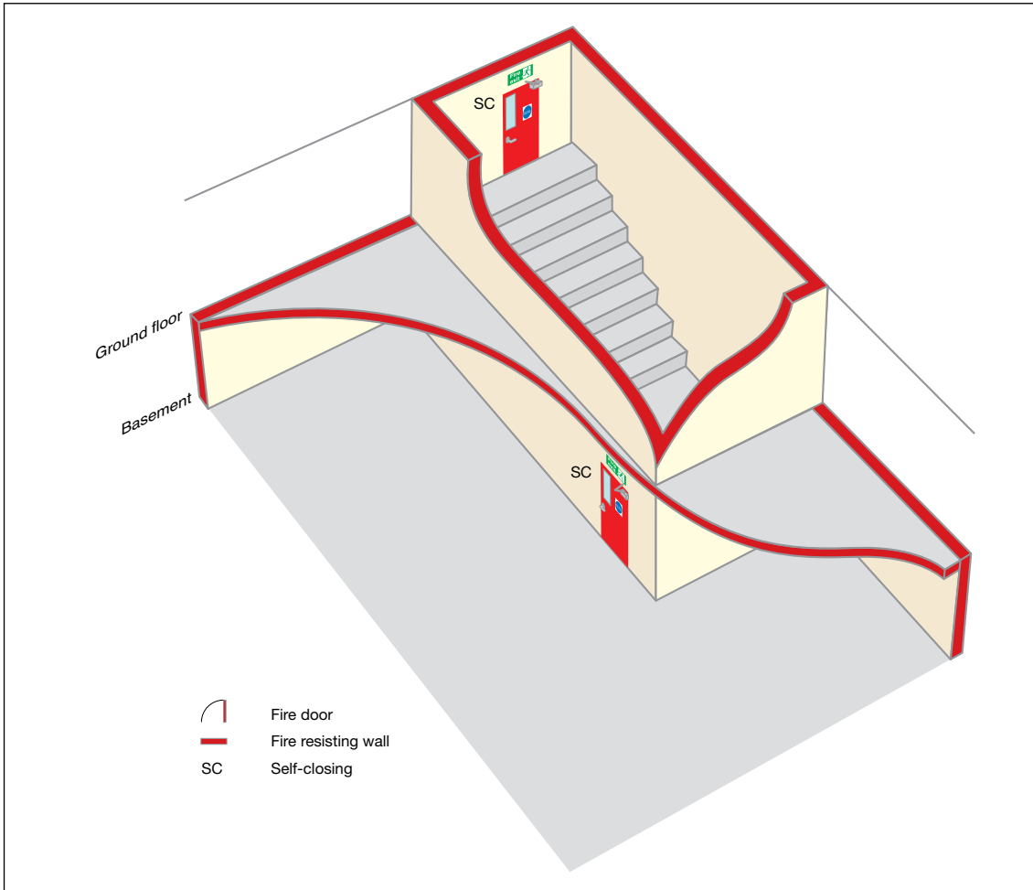
Figure 32: Basement protection
