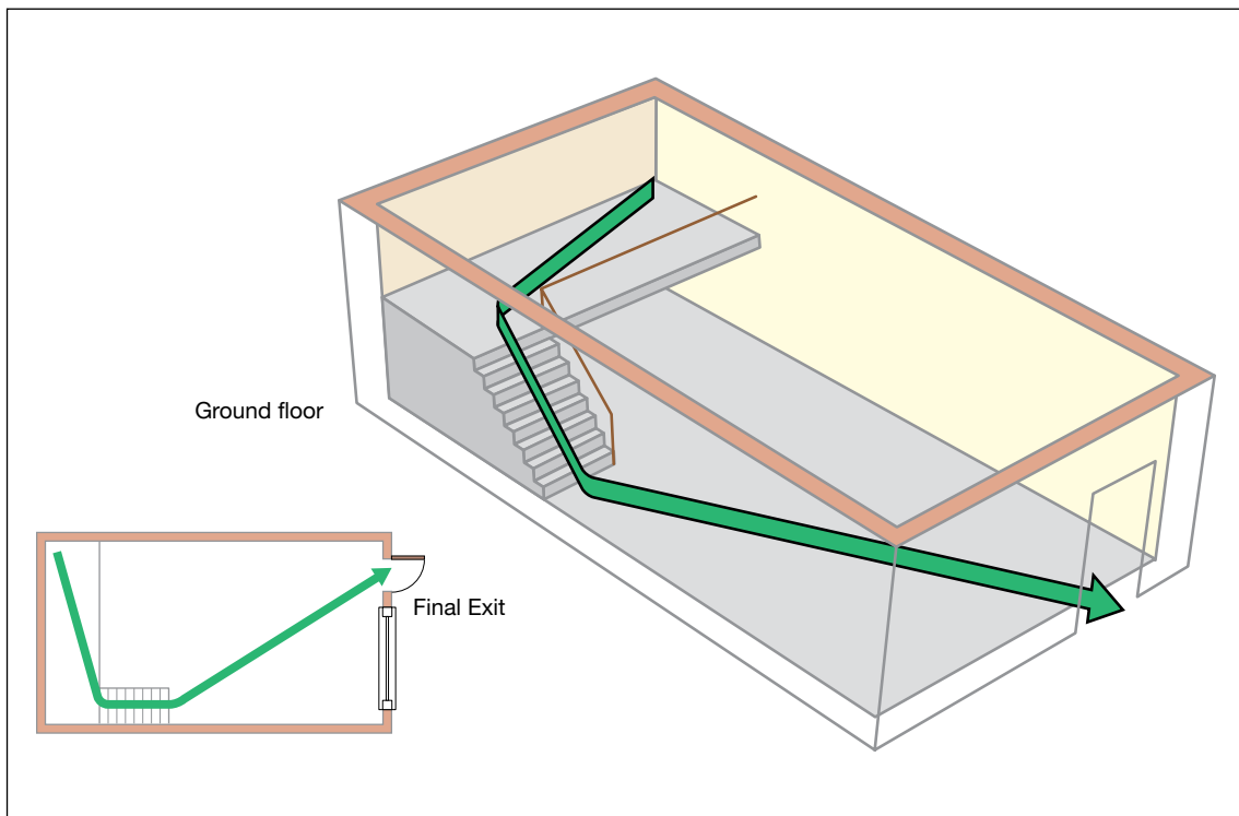
Figure 43: Ground floor with a single exit (including a mezzanine)
