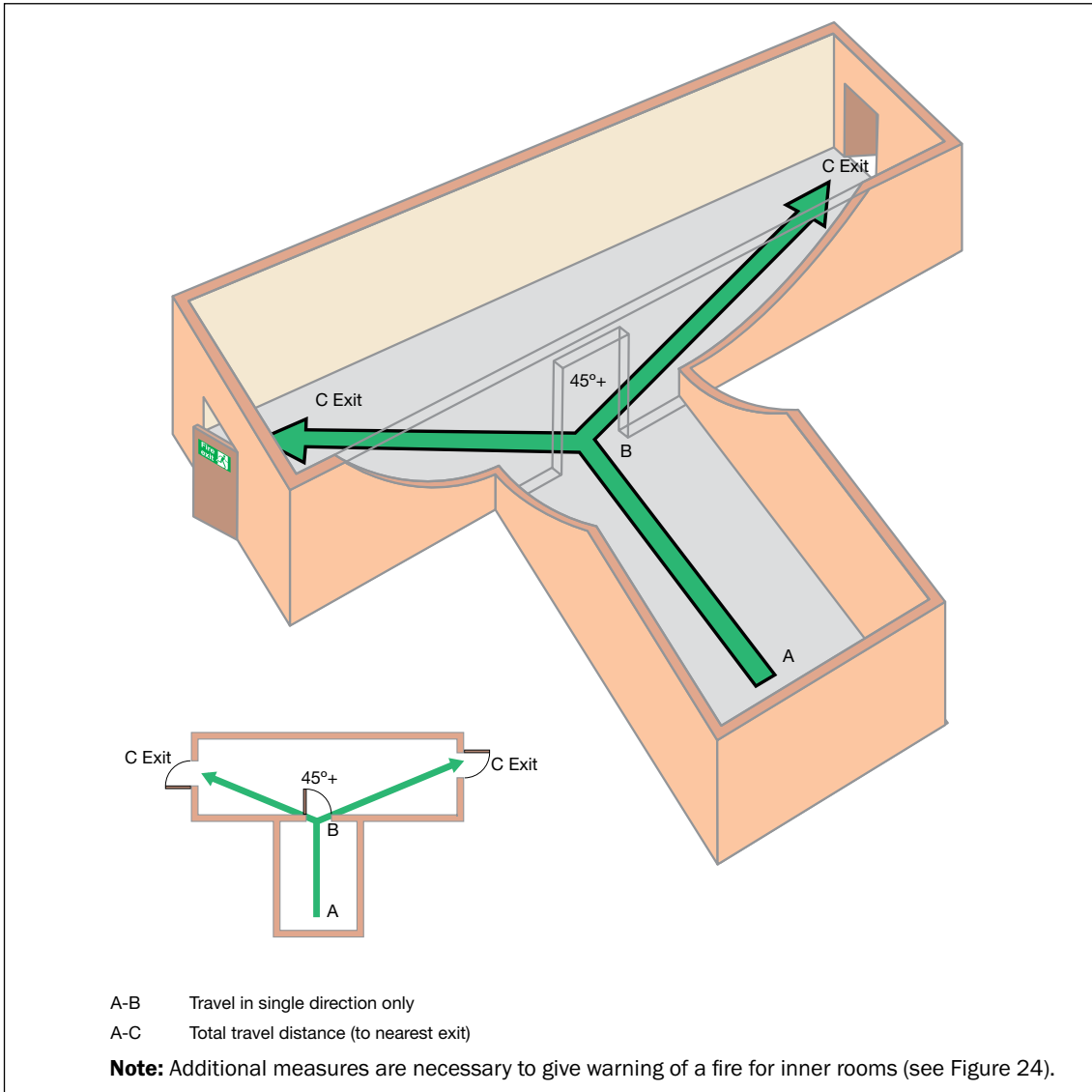
Figure 28: Measuring travel distance from initial dead end (inner room)
